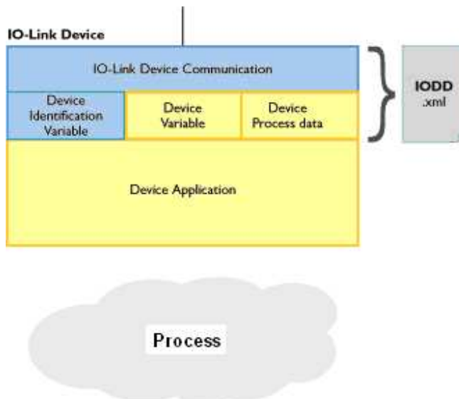
Rysunek 10: IO-Link device structure
